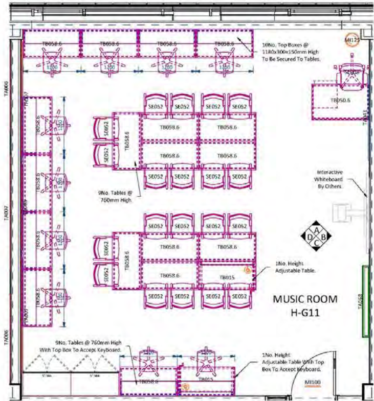
H-G11 Music Room 1 : 50
